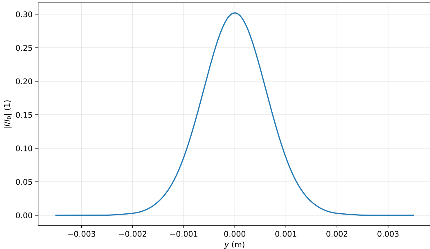
Intensity profile I(x=0, y, z=3.503)/I_0 , P_{in}=0.2P_{cr} , artificial time
